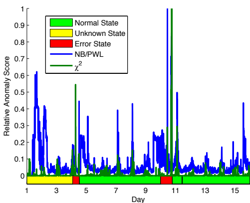
Figure 7. Anomaly scores over time for NB/PWL and \chi^2 on data set 5, “Bad URL and Runaway Query”. The major failures occurred on days 4 and 10.
