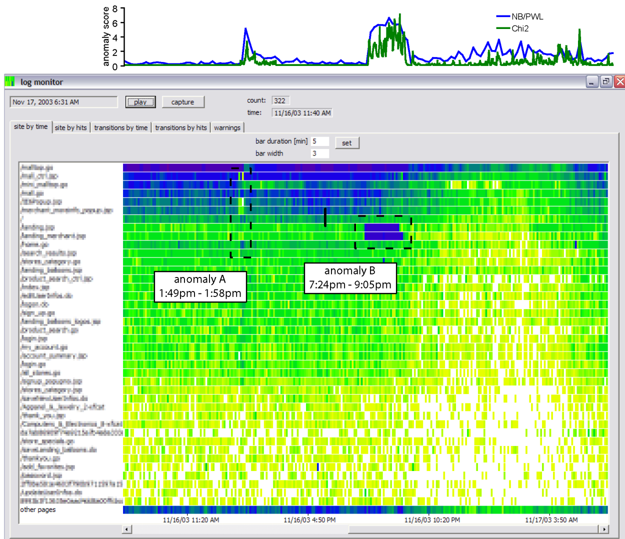
Figure 1. An annotated screen shot of the visualization tool. (Note: if this paper was printed in black-and-white, please see the hi-res color figures at http://www.cs.berkeley.edu/~bodikp/icac05/ . Color is an integral component of the visualization.) The horizontal axis is time in 5-minute intervals. Each horizontal bar represents the hit count to one of the 40 most-requested pages; the bottom bar counts hits to all other pages combined. A blue tile means the corresponding page received > 100 hits during that 5-minute interval; green > 10 hits, yellow > 1 hit, white (no tile) zero hits. The graph on the top shows the corresponding anomaly scores. In this screenshot we clearly see two anomalies from data set 1: A (1:49pm to 1:58pm) and B (7:24pm to 9:05pm).
