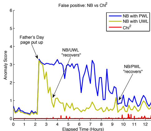
Figure 8. Illustration of a case where the NB algorithms detect a false positive (due to introduction of a new page) but \chi^2 does not.
