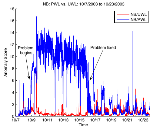
Figure 6. Whereas “careful learner” NB/PWL continues to detect the broken signup page anomaly (data set 3) for all 7 days, “eager learner” NB/UWL quickly decides that this new behavior is normal.
