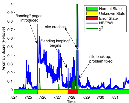
Figure 5. Anomaly scores over time for NB/PWL and \chi^2 on data set 2, “Landing Loop”. The time period from the introduction of the landing pages until Ebates’ detection of the landing loop problem is marked as unknown, since we haven’t been able to determine with 100% certainty whether this time period was problematic for Ebates or not.
