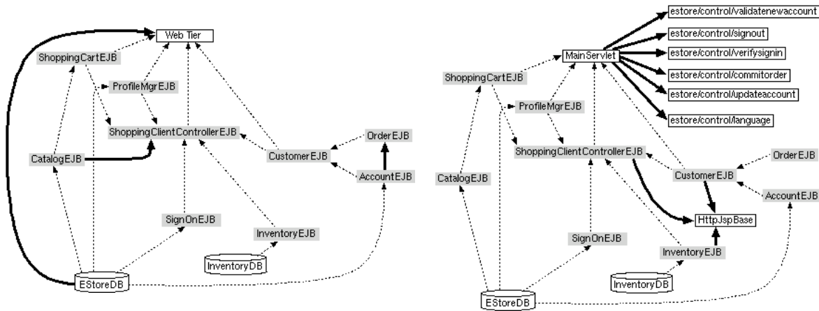
Figure 2. Two f-maps for Petstore: one obtained through manual inspection of deployment descriptors (left) and one obtained automatically by our introspective system (right). The bold edges are those that are not common between the two f-maps.
