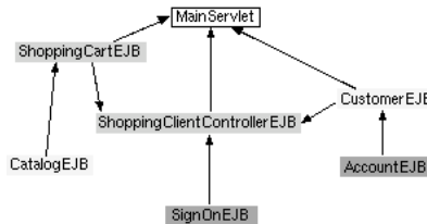
Figure 4. Petstore f-map based exclusively on application-declared exceptions.
